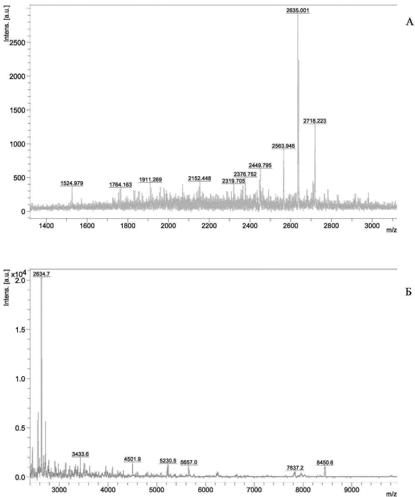
Figure 1. Mass spectrum of cortexin peptides. A is the mass range of 1400-3000 Da, B is the mass range of 3000-10000 Da.
